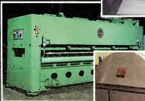
Fehrer —Needle looms with speeds to 2300 strokes/min. and widths to 257". Nonwoven web forming plants with widths to 213".
